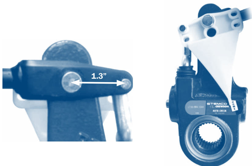
STEMCO Crewson Automatic Brake Adjuster
